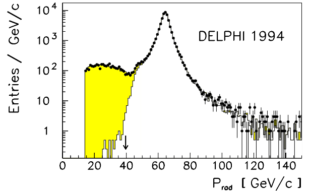
Fig. 8. Distribution of the event variable P_{rad} for data from the 1994 running period (points) and the fitted Monte Carlo. The unshaded area is the contribution from \mu^+\mu^- , and the shaded area is the contribution from \tau^+\tau^- . The arrow indicates the cut applied in the final event selection
