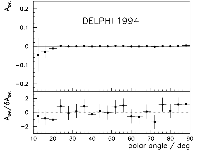
Fig. 10. Muon detection asymmetry A_{det} versus the polar angle as determined for the 1994 running period, both as an absolute quantity, and normalized by its statistical uncertainty, \delta A_{det}
