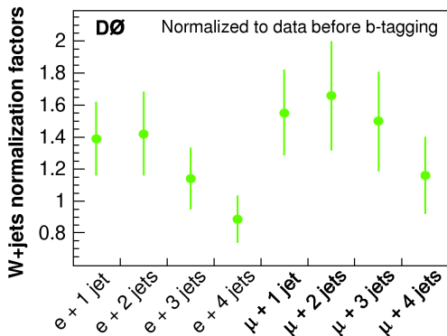
FIG. 4: The factors used to normalize the W +jets background model to pretagged data in each analysis channel.
