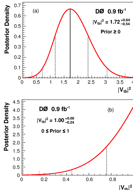
FIG. 30: The posterior density distributions for |V_{tb}|^2 for (a) a nonnegative flat prior, and (b) a flat prior restricted to the region [0, 1] and assuming f_1^L = 1 . The dashed lines show the positions of the one, two, and three standard deviation distances away from the peak of each curve.
