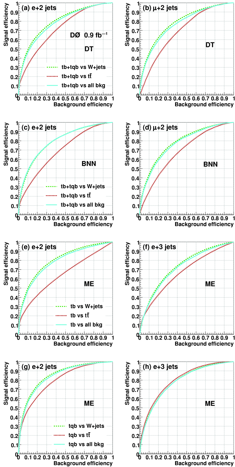
FIG. 14: For plots (a)–(d), DT and BNN tb+tqb signal efficiency versus background efficiency in the e +jets channel (left column) and \mu +jets channel (right column) for events with two jets of which one is b tagged. Plots (e)–(h) show the ME signal versus background efficiency for tb signal (third row) and tqb signal (fourth row), for b tagged e +jets events with two jets (left column) and three jets (right column). These curves are derived from the discriminants shown in Fig. 13.
