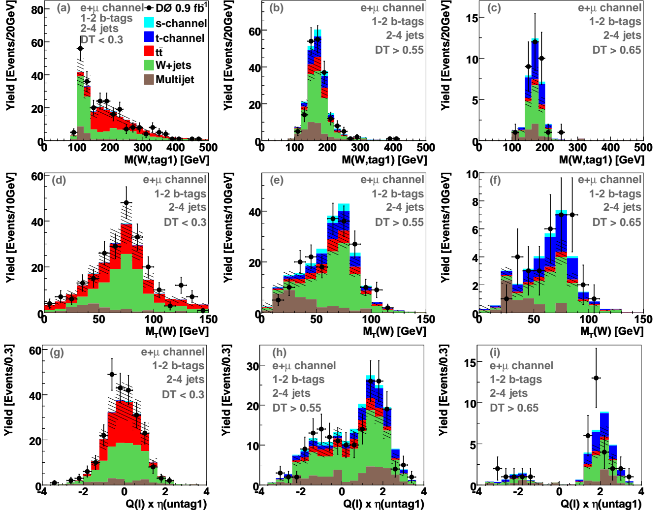
FIG. 24: The b -tagged top quark mass (top row), W boson transverse mass (second row) and Q(\text{lepton}) \times \eta(\text{untag1}) (third row) for the t\bar{b}+tq\bar{b} analysis with a low ( < 0.3 , left column), high ( > 0.55 , middle column), and very high ( > 0.65 , right column) DT output, for lepton flavor ( e, \mu ), number of b -tagged jets (1,2), and jet multiplicity (2,3,4) combined. Hatched areas represent the systematic and statistical uncertainties on the background model. The signal cross section is the measured one (4.9 pb).
