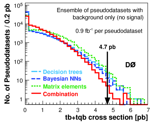
FIG. 28: Distributions of the cross sections measured from data by the three analyses and their combination, using the background-only ensemble. The arrow shows the combined cross section measurement, 4.7 pb.
