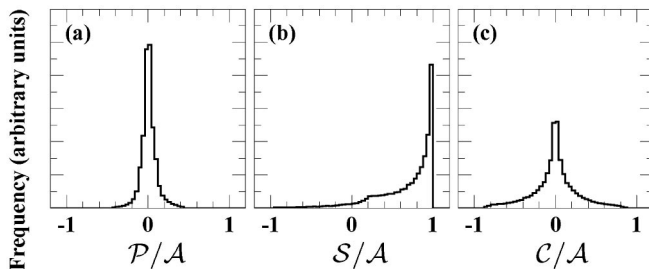
FIG. 2. (a) The distribution of \mathcal{P}(\omega; \mathbf{A})/\mathcal{A}(\omega; \mathbf{A}) , (b) S(\omega; \mathbf{A})/\mathcal{A}(\omega; \mathbf{A}) and (c) C(\omega; \mathbf{A})/\mathcal{A}(\omega; \mathbf{A}) , where \mathcal{A} , \mathcal{P} , S and C are defined by Eq. (14), for a set of events generated according to the amplitudes \mathbf{A} corresponding to the BABAR values in Table I.
