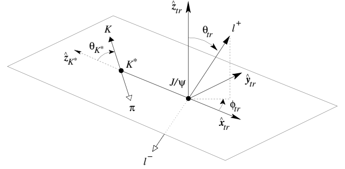
FIG. 1. Definition of the transversity angles ( \theta_{K^*}, \theta_{lr}, \phi_{lr} ) and coordinate system ( \hat{x}_{lr}, \hat{y}_{lr}, \hat{z}_{lr} ). The direction opposite to the B meson momentum in the J/\psi rest frame is \hat{x}_{lr} ; \hat{y}_{lr} is perpendicular to \hat{x}_{lr} in the plane that contains \hat{x}_{lr} and \vec{p}_K , chosen so \vec{p}_K \cdot \hat{y}_{lr} > 0 ; \hat{z}_{lr} = \hat{x}_{lr} \times \hat{y}_{lr} . The helicity angle \theta_{K^*} of the K^* decay is the angle between the direction opposite to the B meson flight direction and the kaon momentum, in the K^* rest frame. Finally, \theta_{lr} and \phi_{lr} are the polar and azimuthal angle of the positive lepton defined in the J/\psi rest frame.
